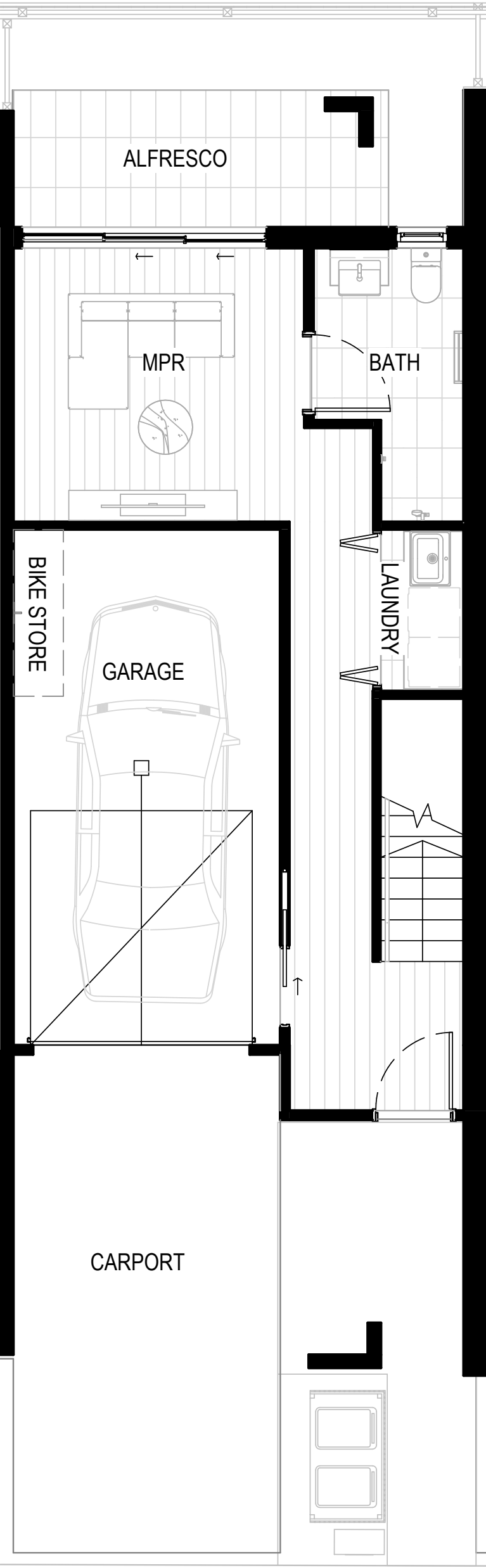
Ground Floor
