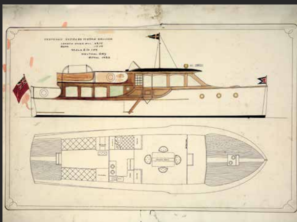
1938 — Proposed 30 foot Harbour launch Australian National Maritime Museum Collection Gift from Harvey Halvorsen and Judith Lynn Vigo
