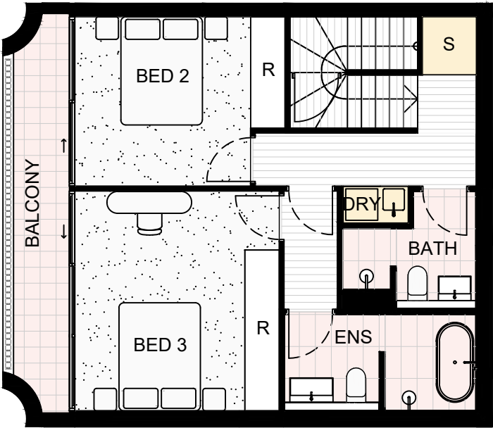
LEVEL 01
